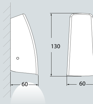
WALL INSTALLATION
