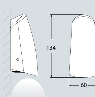
WALL INSTALLATION
