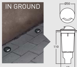
IN GROUND
