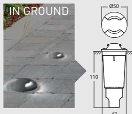
IN GROUND
