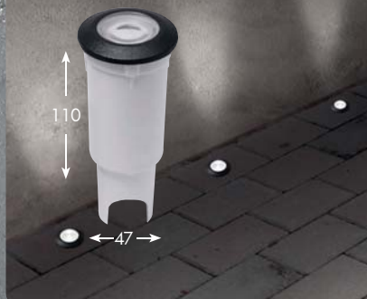
IN GROUND INSTALLATION
